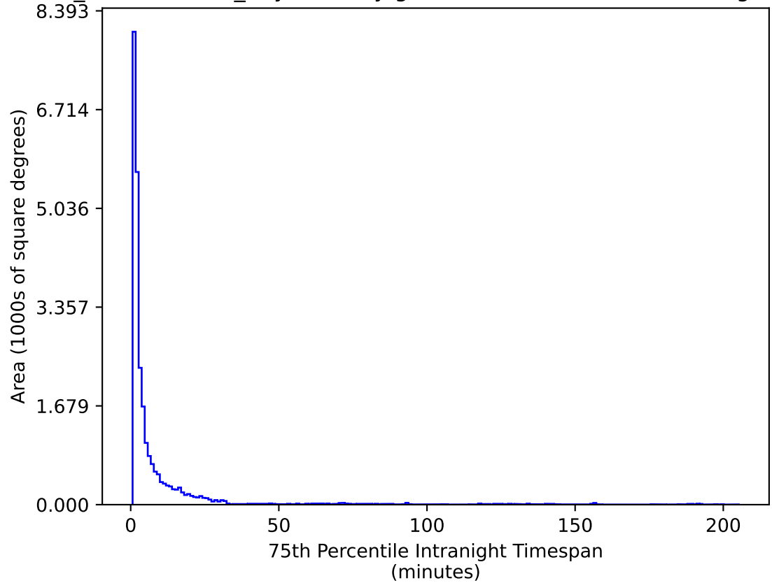
weather_cloudso4v3.4_10yrs All sky g band: 75th Percentile Intranight Timespan
