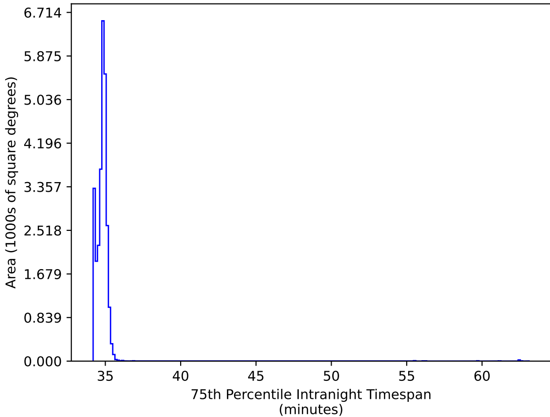
weather_cloudso4v3.4_10yrs All sky: 75th Percentile Intranight Timespan
