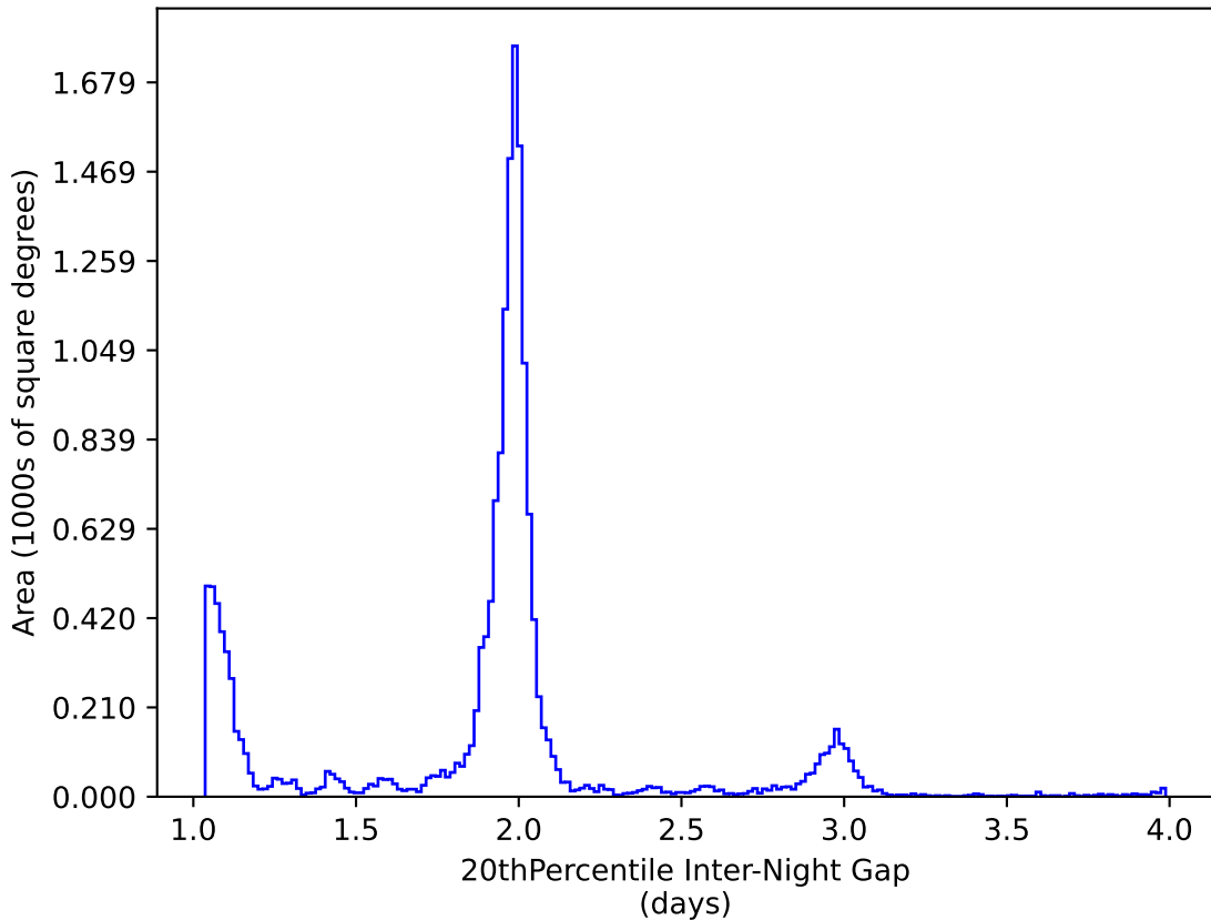
weather_cloudso4v3.4_10yrs WFD y band: 20thPercentile Inter-Night Gap
