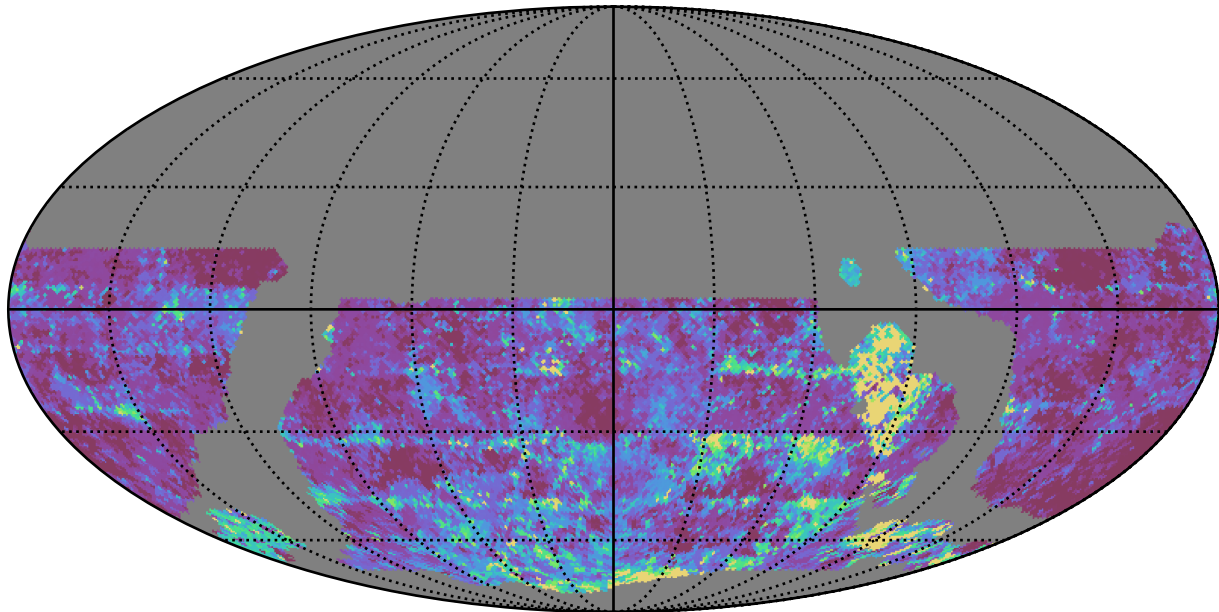
weather_cloudso4v3.4_10yrs WFD u band: 20thPercentile Inter-Night Gap
