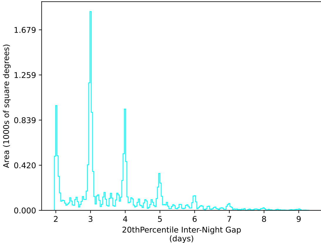
weather_cloudso4v3.4_10yrs WFD u band: 20thPercentile Inter-Night Gap
