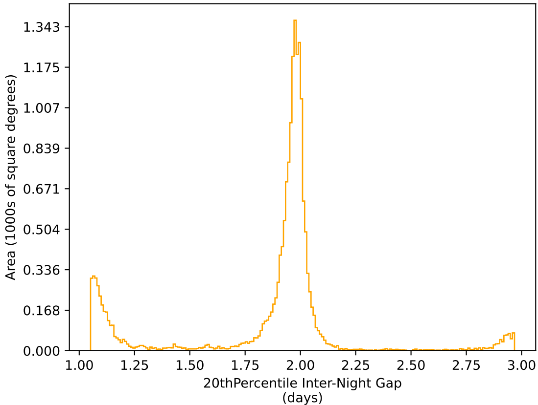
weather_cloudso4v3.4_10yrs WFD r band: 20thPercentile Inter-Night Gap
