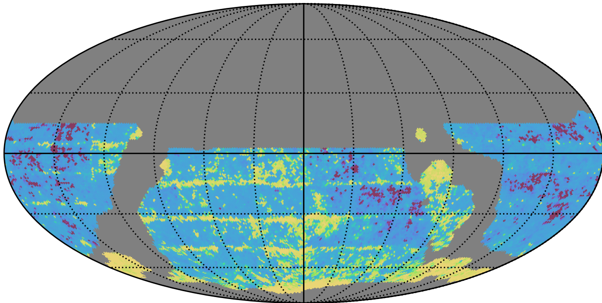
weather_cloudso4v3.4_10yrs WFD i band: 20thPercentile Inter-Night Gap
