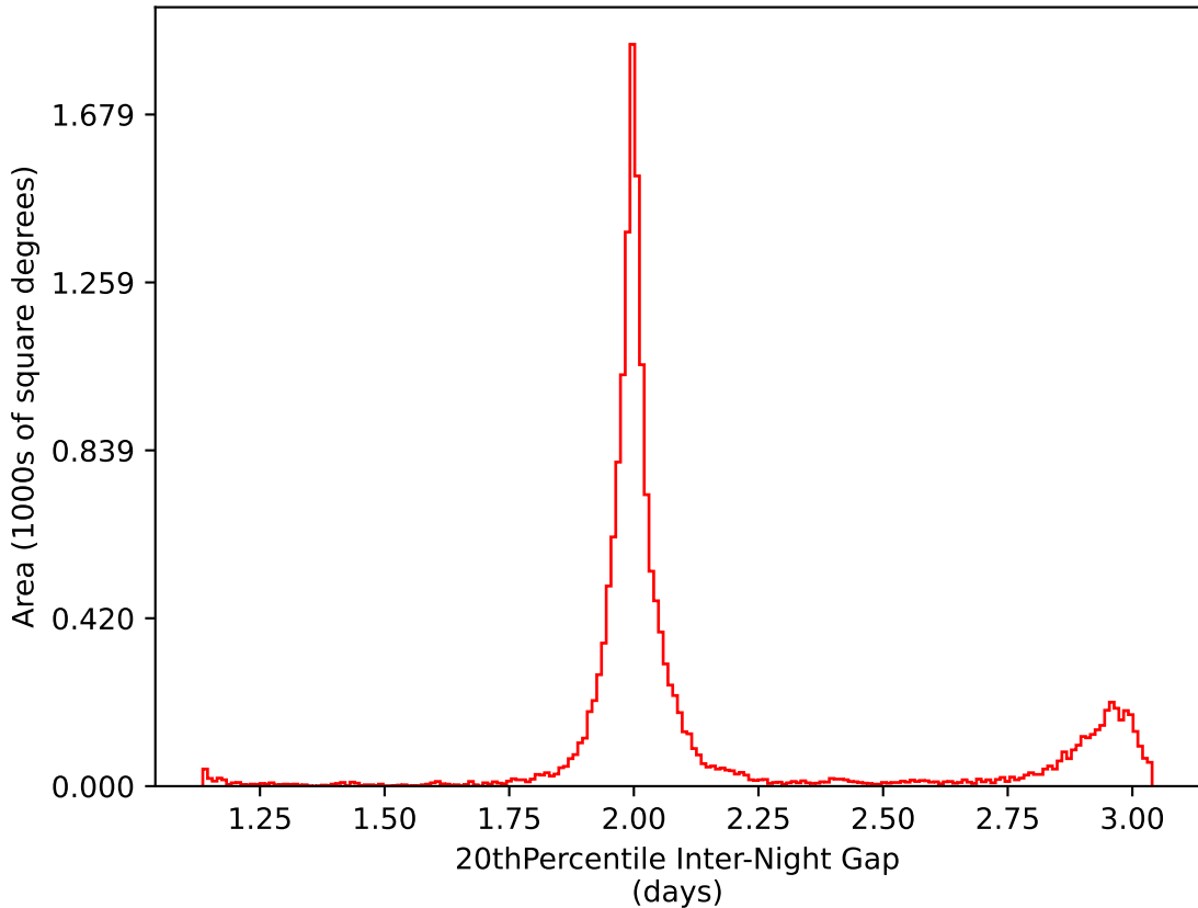
weather_cloudso4v3.4_10yrs WFD i band: 20thPercentile Inter-Night Gap
