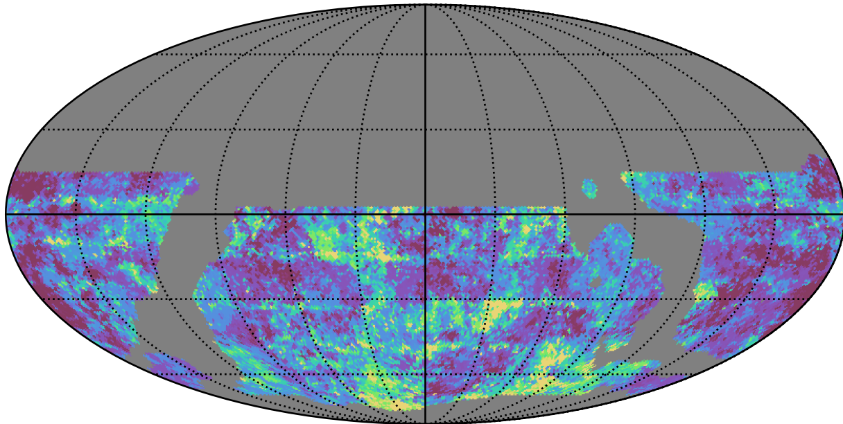
weather_cloudso4v3.4_10yrs WFD g band: 20thPercentile Inter-Night Gap
