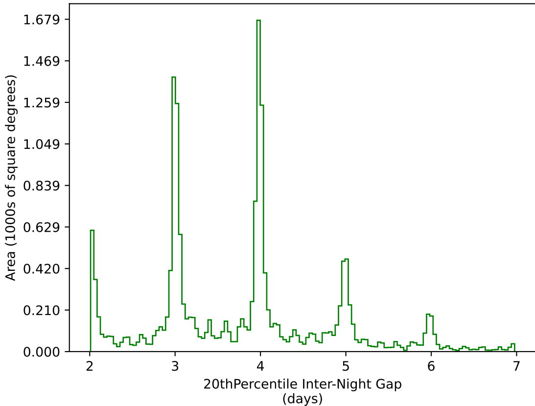
weather_cloudso4v3.4_10yrs WFD g band: 20thPercentile Inter-Night Gap
