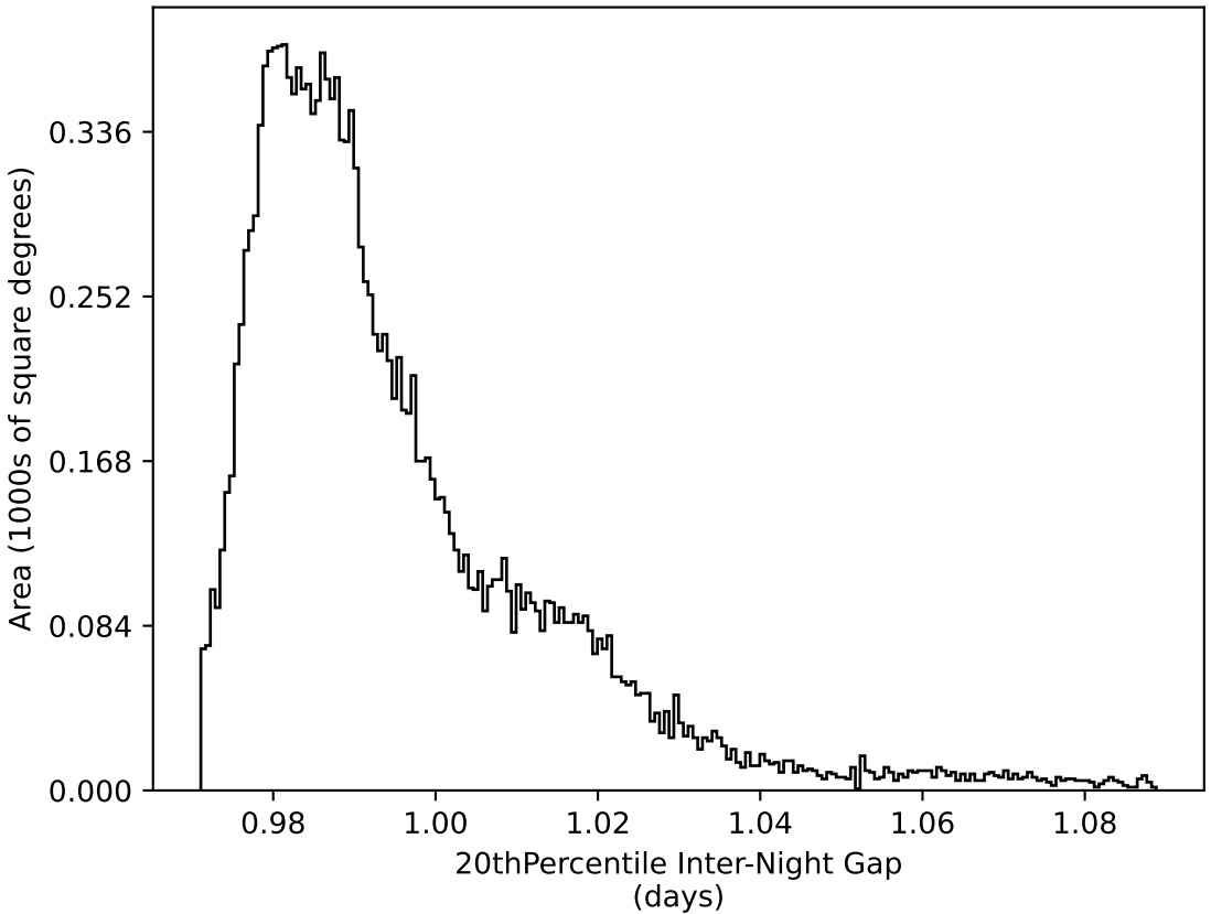
weather_cloudso4v3.4_10yrs WFD all bands: 20thPercentile Inter-Night Gap
