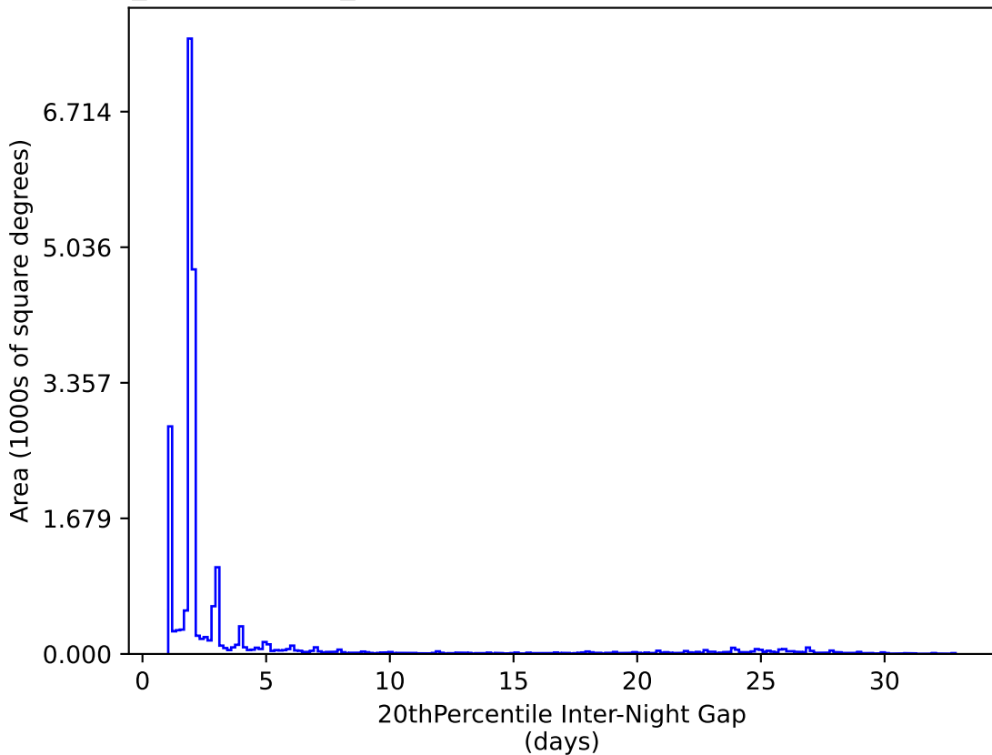
weather_cloudso4v3.4_10yrs All sky y band: 20thPercentile Inter-Night Gap
