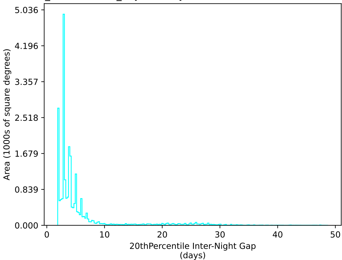
weather_cloudso4v3.4_10yrs All sky u band: 20thPercentile Inter-Night Gap
