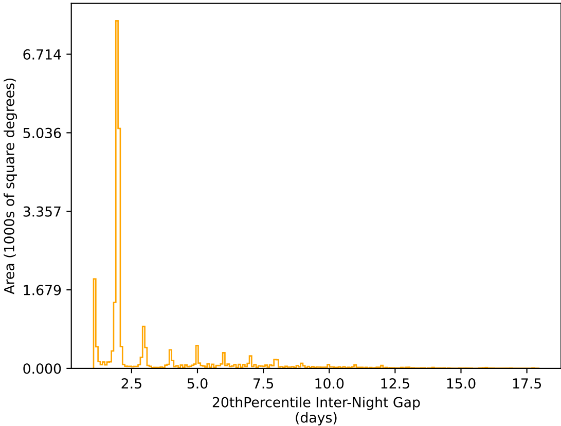
weather_cloudso4v3.4_10yrs All sky r band: 20thPercentile Inter-Night Gap
