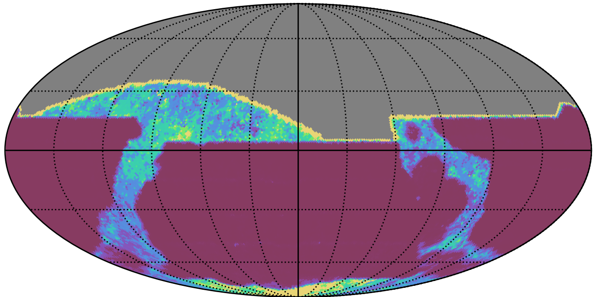
weather_cloudso4v3.4_10yrs All sky all bands: 20thPercentile Inter-Night Gap
