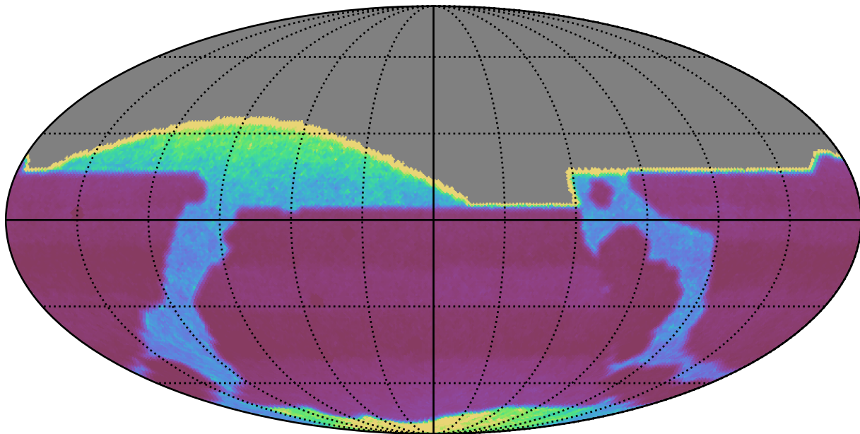
weather_cloudso4v3.4_10yrs : properMotion
