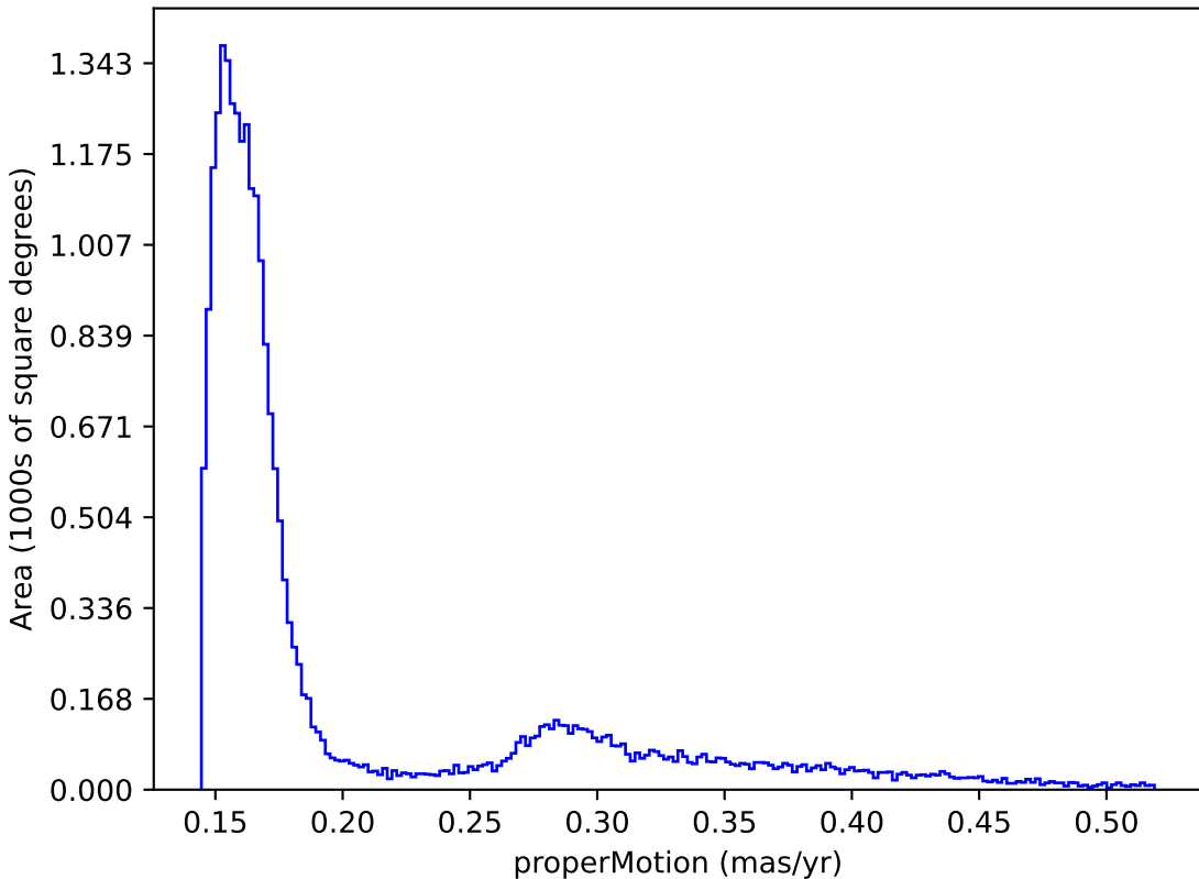
weather_cloudso4v3.4_10yrs : properMotion
