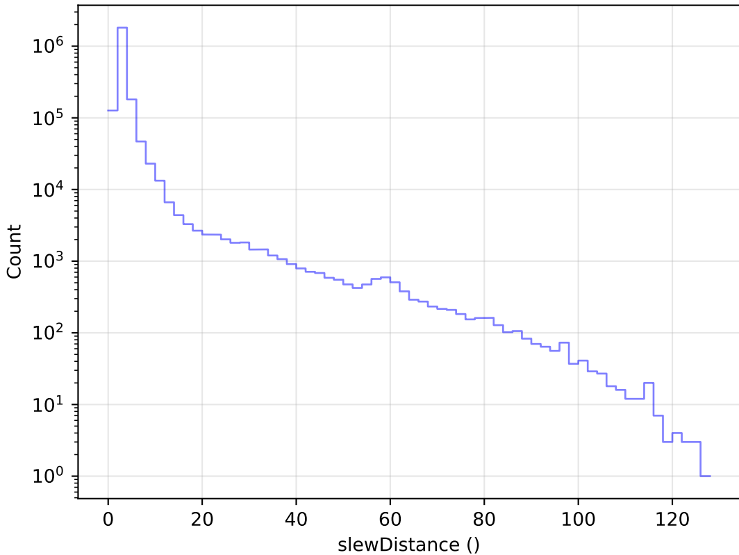
weather_cloudso4v3.4_10yrs All visits: Slew Distance Histogram
