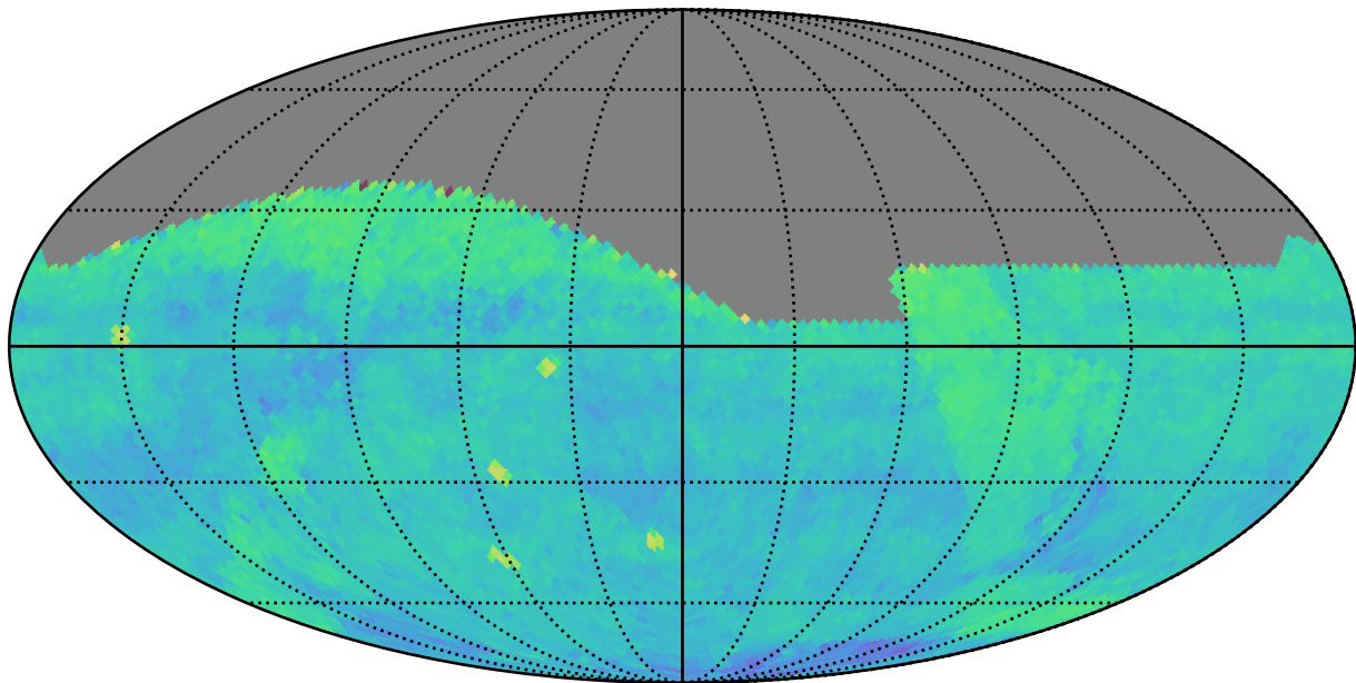
weather_cloudso4v3.4_10yrs (g or r or i): PairFraction
