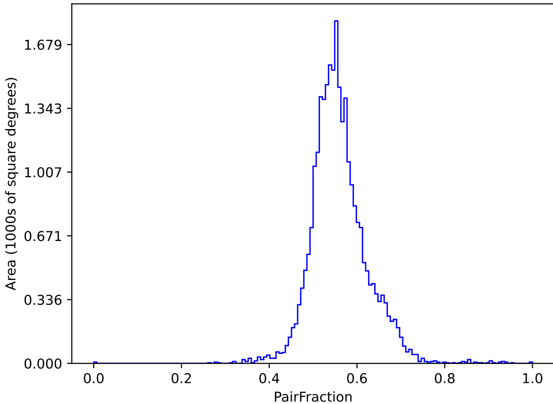
weather_cloudso4v3.4_10yrs (g or r or i): PairFraction
