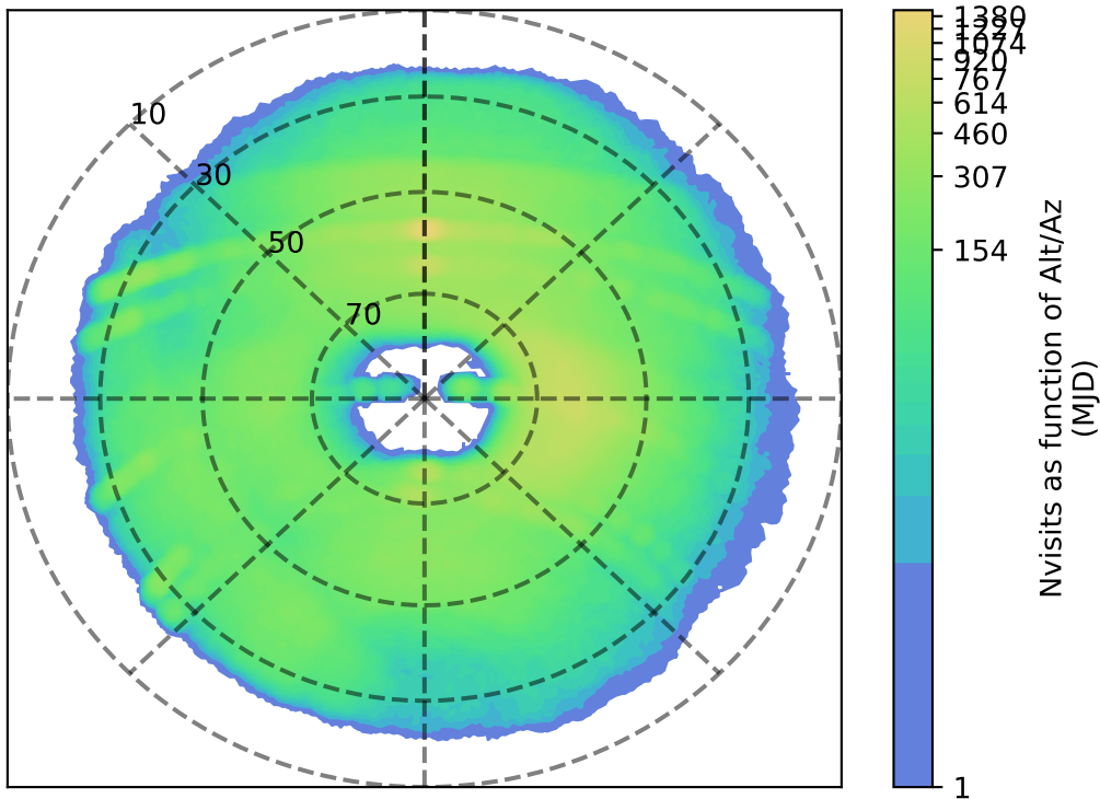
weather_cloudso4v3.4_10yrs g: Nvisits as function of Alt/Az
