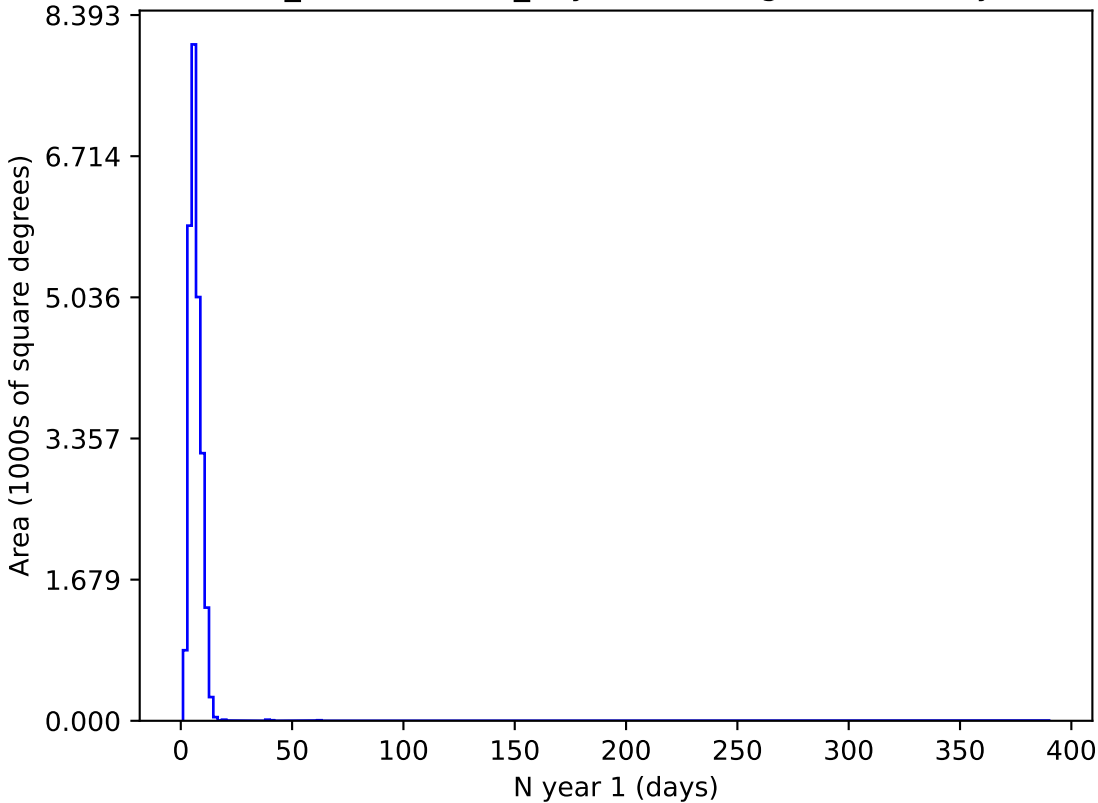
weather_cloudso4v3.4_10yrs u and night &lt; 365: N year 1
