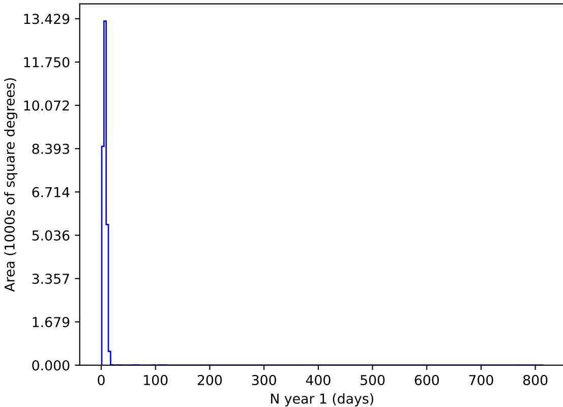
weather_cloudso4v3.4_10yrs g and night < 365: N year 1
