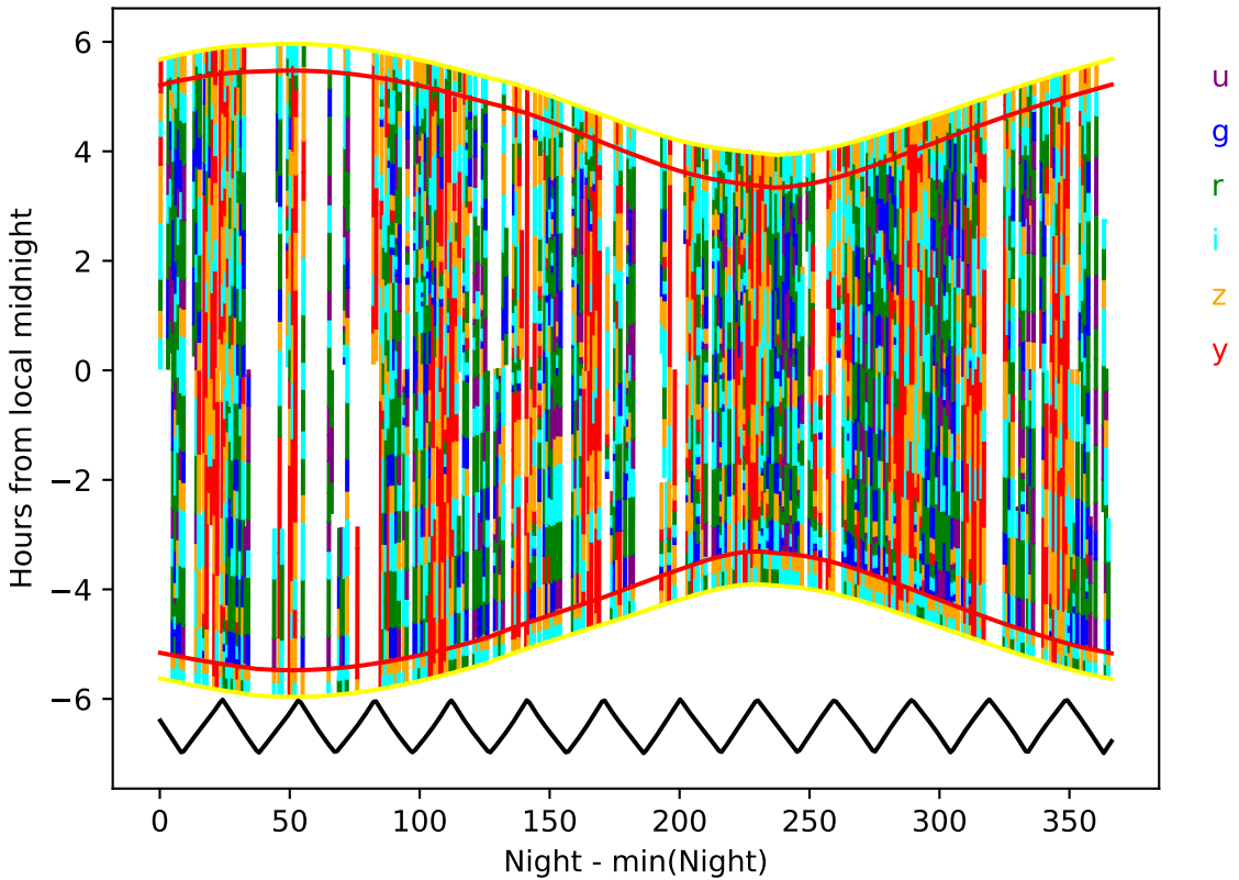
weather_cloudso4v3.4_10yrs year 7-8: Hourglass
