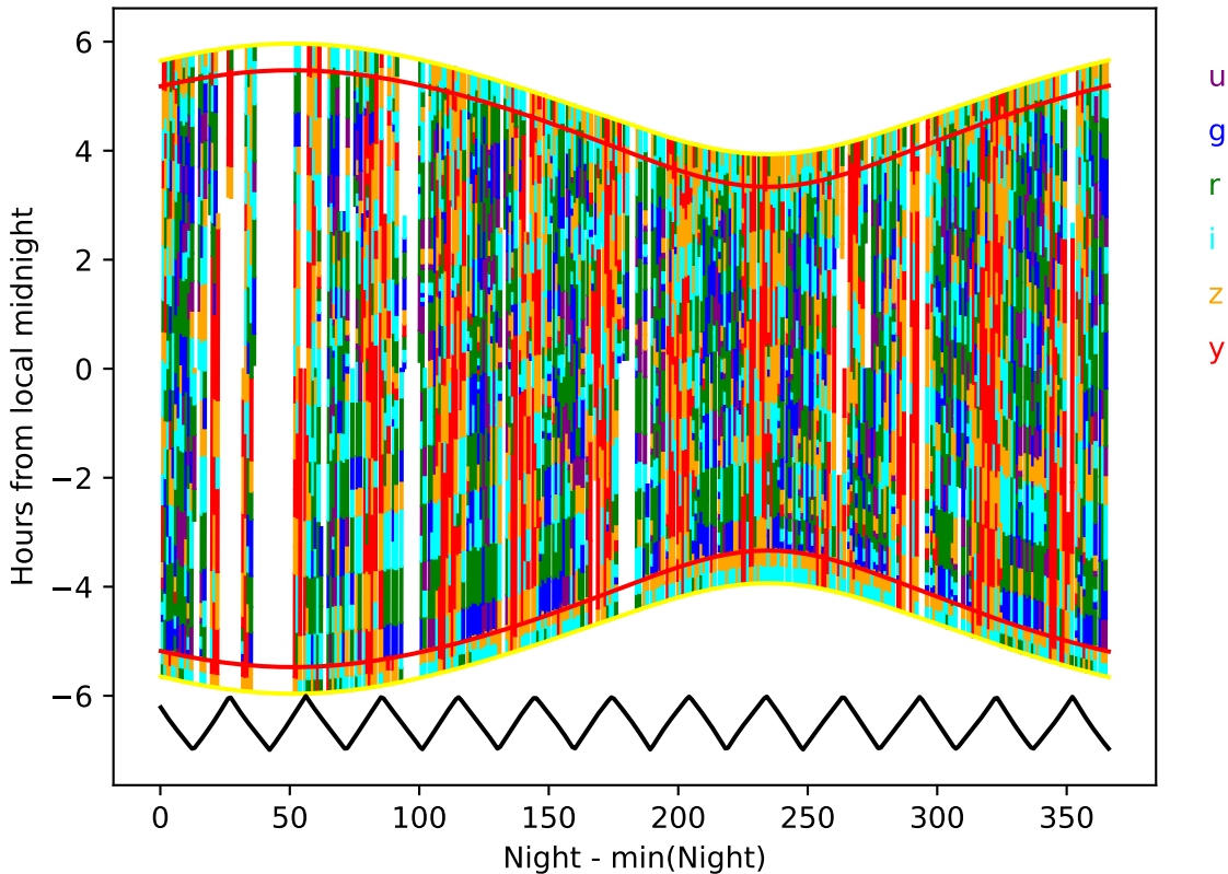
weather_cloudso4v3.4_10yrs year 4-5: Hourglass
