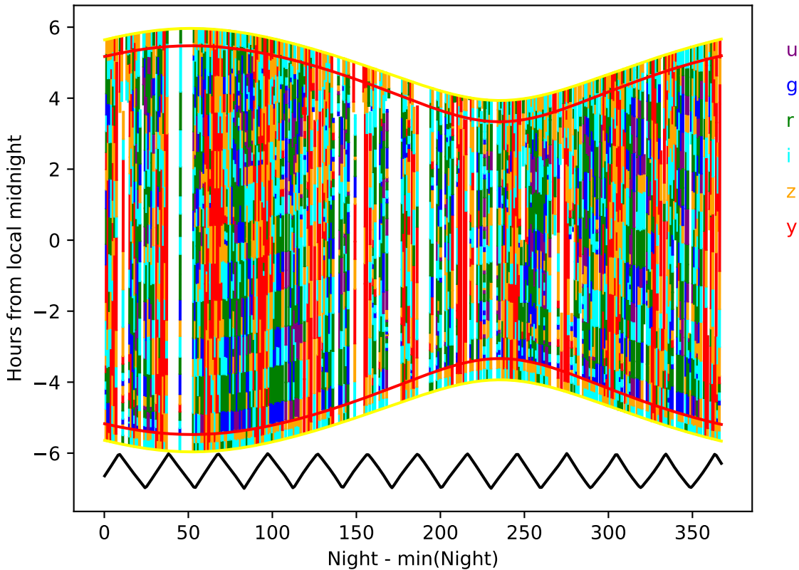
weather_cloudso4v3.4_10yrs year 3-4: Hourglass
