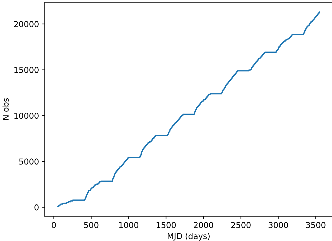
weather_cloudso4v3.4_10yrs note like DD:ELAISS1%: Cumulative
