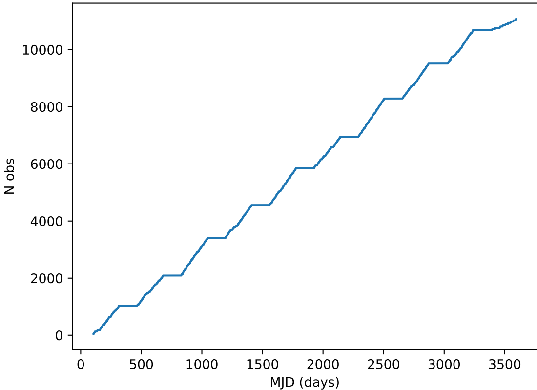
weather_cloudso4v3.4_10yrs note like DD:EDFS_b%: Cumulative
