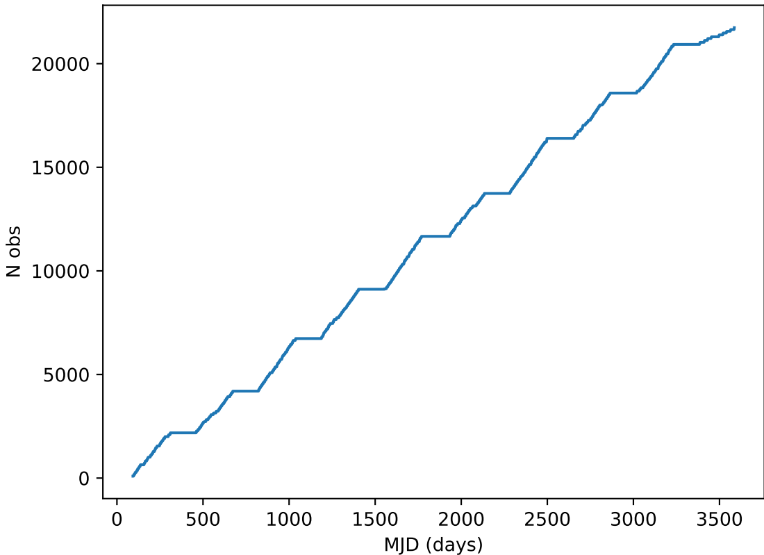
weather_cloudso4v3.4_10yrs note like DD:ECDFS%: Cumulative
