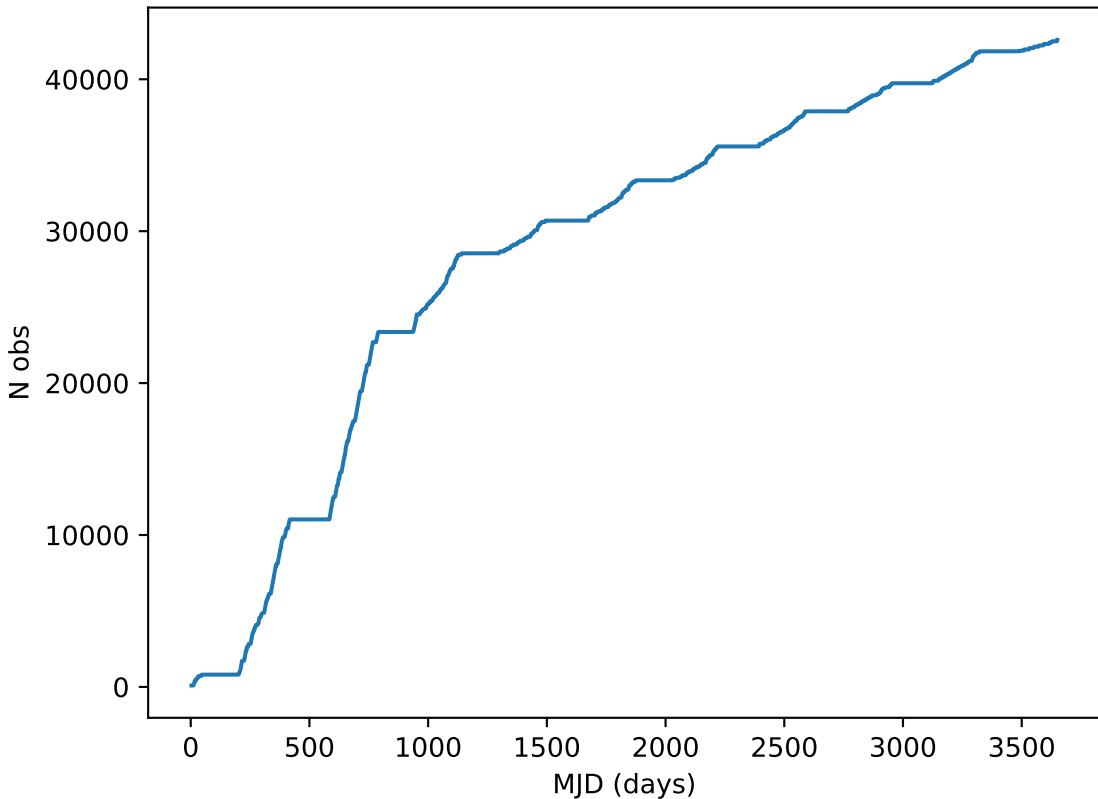
weather_cloudso4v3.4_10yrs note like DD: COSMOS%: Cumulative
