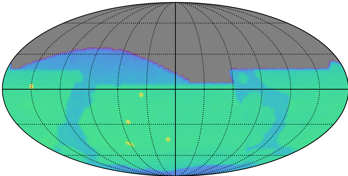
weather_cloudso4v3.4_10yrs z: CoaddM5
