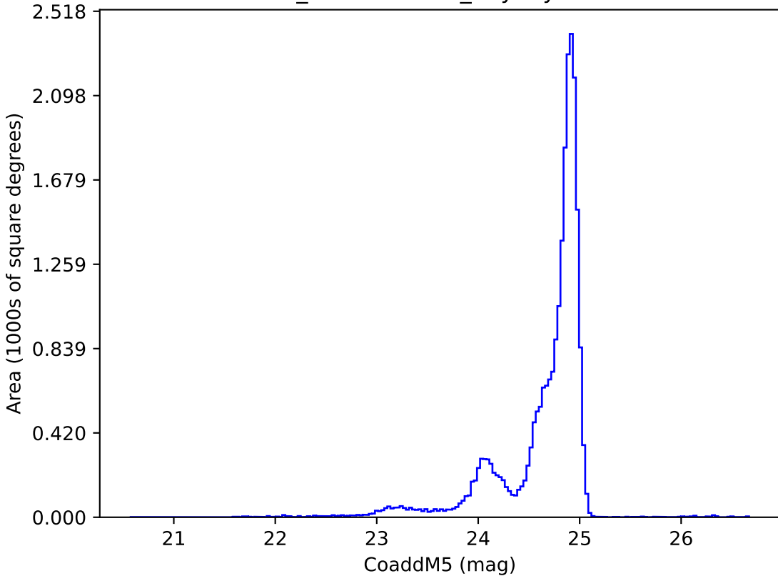
weather_cloudso4v3.4_10yrs y: CoaddM5
