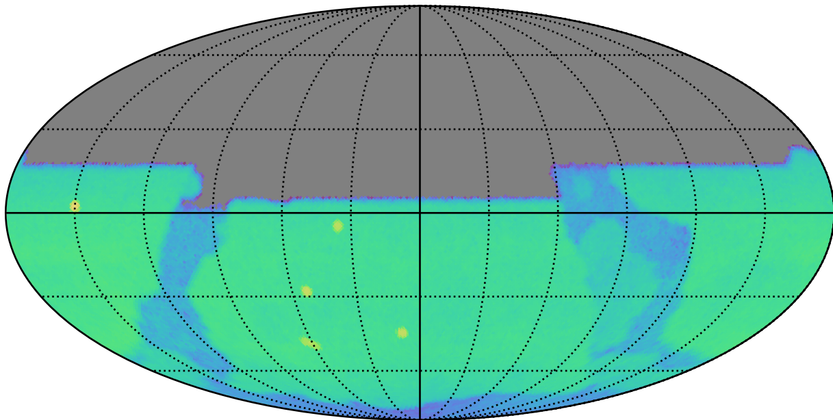
weather_cloudso4v3.4_10yrs u: CoaddM5
