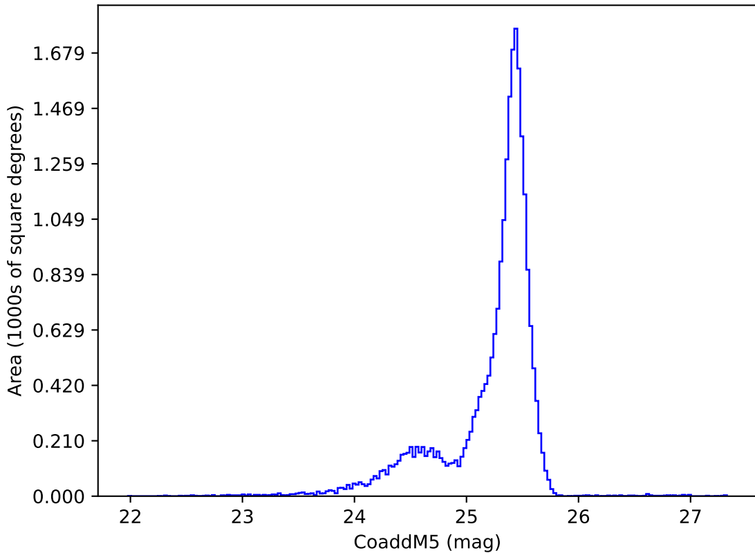
weather_cloudso4v3.4_10yrs u: CoaddM5
