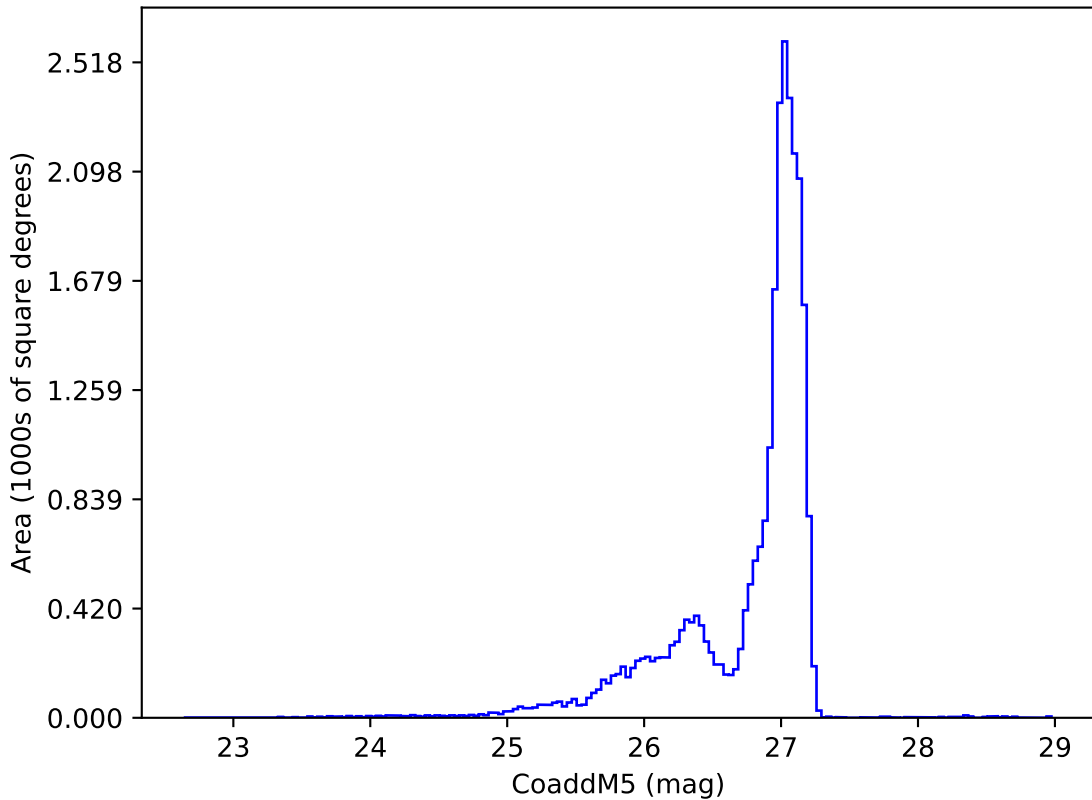
weather_cloudso4v3.4_10yrs r: CoaddM5
