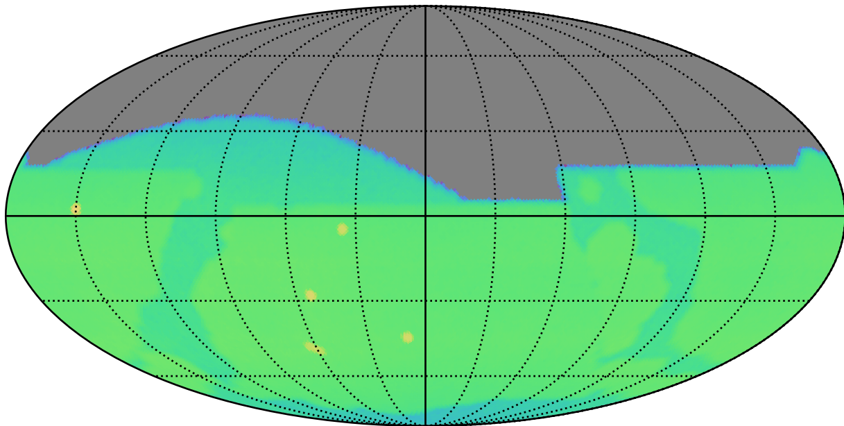
weather_cloudso4v3.4_10yrs : CoaddM5
