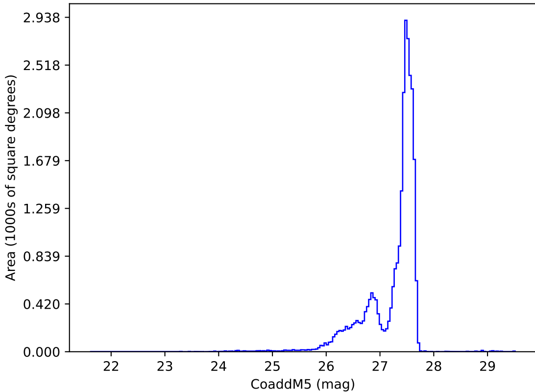
weather_cloudso4v3.4_10yrs : CoaddM5
