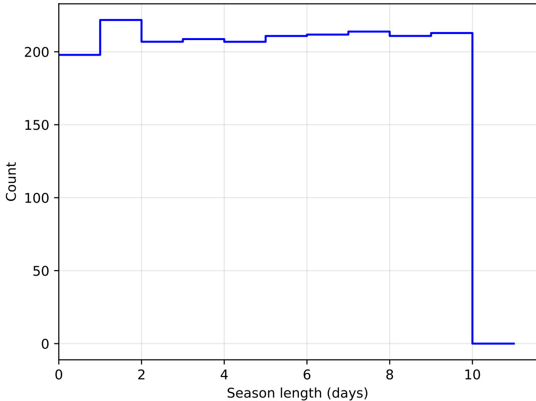
weather_cloudso4v3.4_10yrs DD:ELAISS1 all bands: SeasonLength
