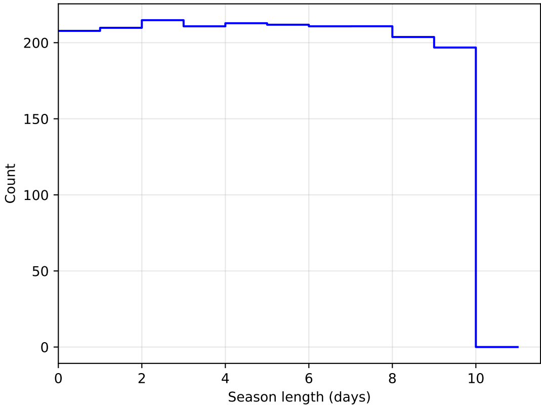
weather_cloudso4v3.4_10yrs DD:EDFS all bands: SeasonLength
