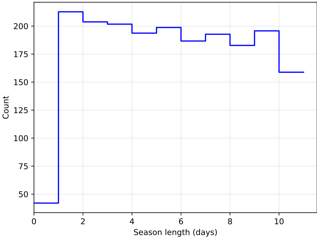
weather_cloudso4v3.4_10yrs DD: COSMOS all bands: SeasonLength
