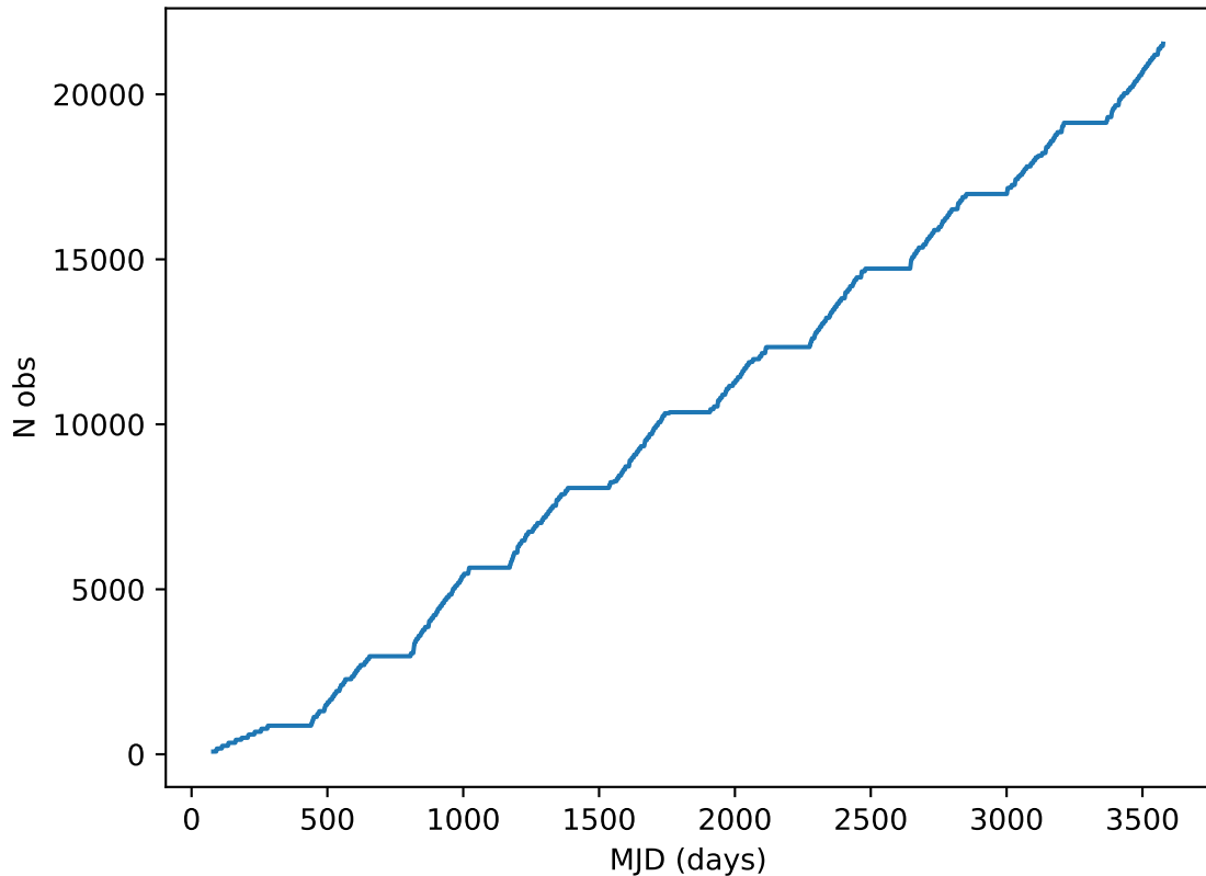
weather_cloudso4v3.4_10yrs all bands: DD:XMM_LSS Cumulative NVisits
