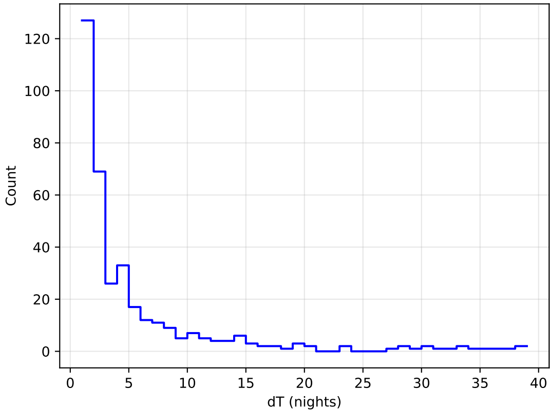
weather_cloudso4v3.4_10yrs all bands: DD:WFD Delta Nights Histogram
