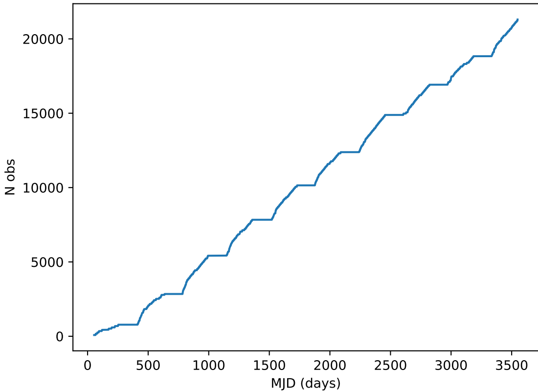
weather_cloudso4v3.4_10yrs all bands: DD:ELAISS1 Cumulative NVisits
