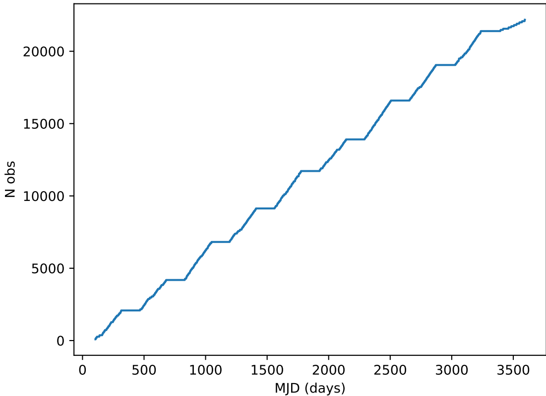
weather_cloudso4v3.4_10yrs all bands: DD:EDFS Cumulative NVisits
