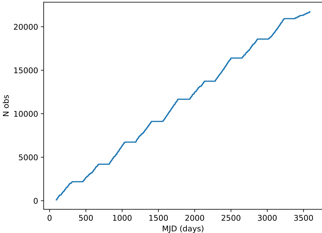
weather_cloudso4v3.4_10yrs all bands: DD:ECDFS Cumulative NVisits
