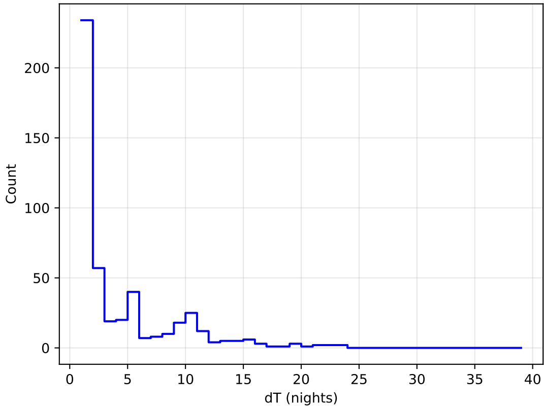
weather_cloudso4v3.4_10yrs all bands: DD: COSMOS Delta Nights Histogram
