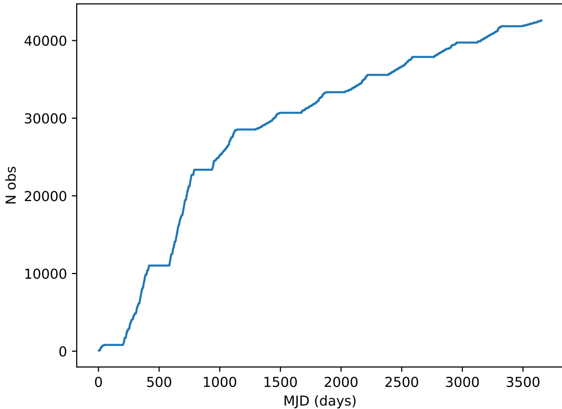
weather_cloudso4v3.4_10yrs all bands: DD: COSMOS Cumulative NVisits
