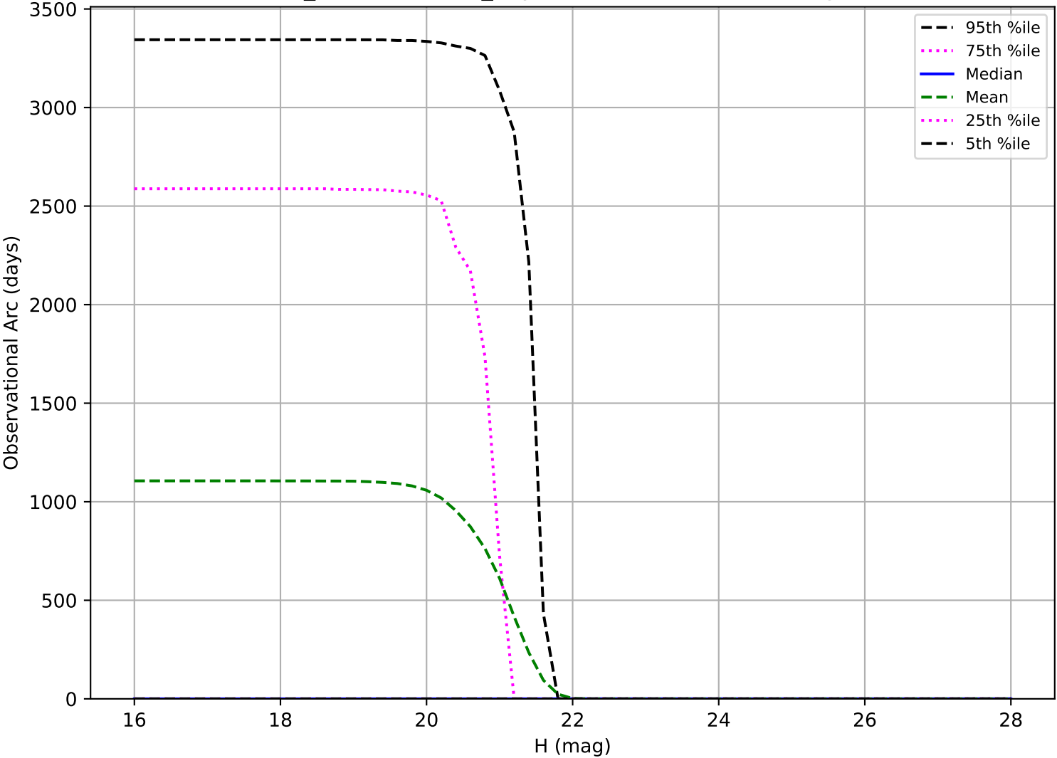
weather_cloudso36v3.4_10yrs: Observational Arc Length Vatra
