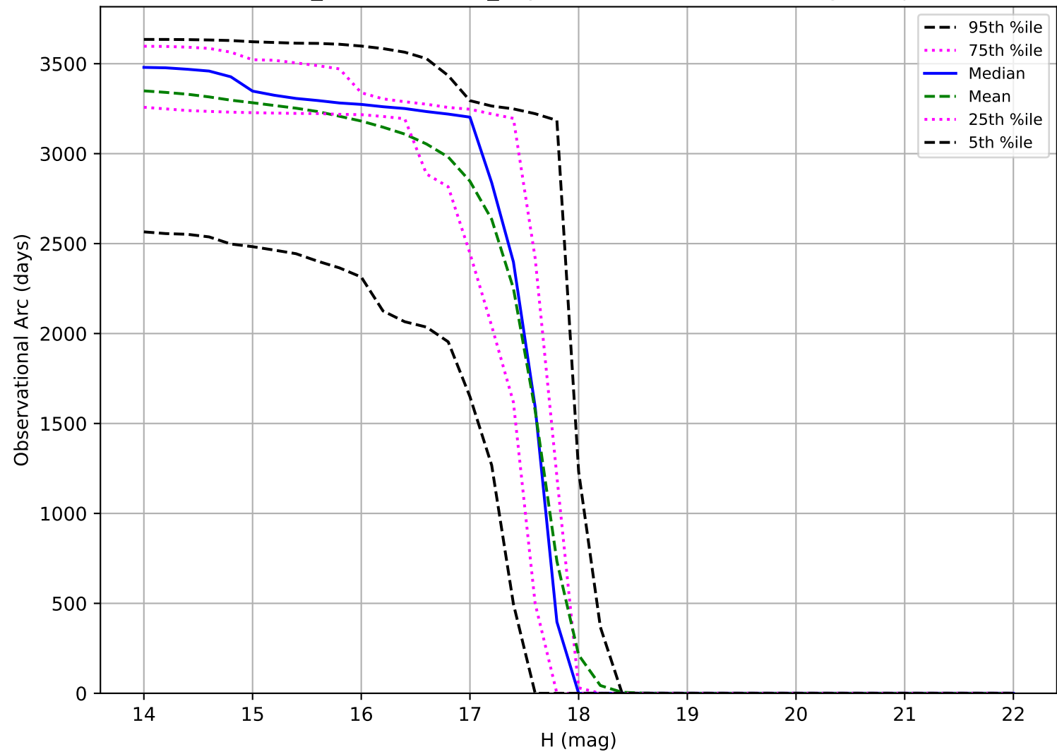
weather_cloudso36v3.4_10yrs: Observational Arc Length Trojan
