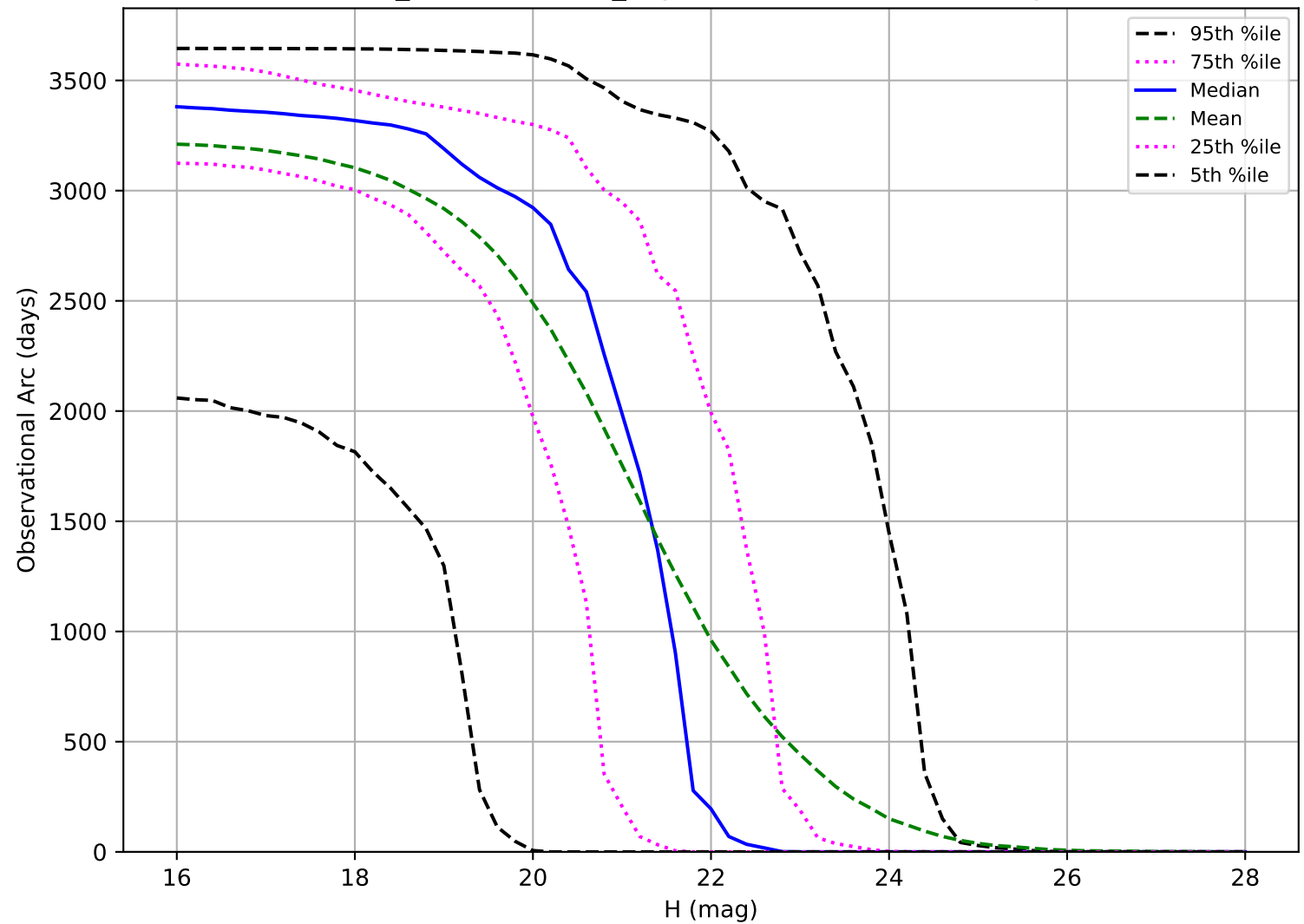
weather_cloudso36v3.4_10yrs: Observational Arc Length PHA
